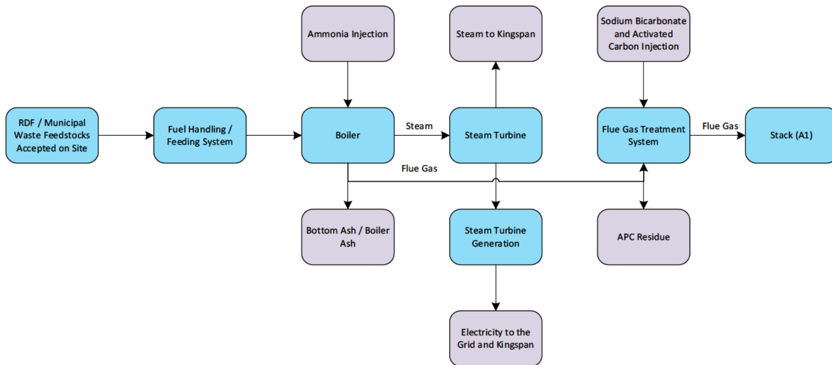
Figure 3.1 – Process Schematic
